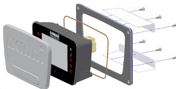
SI-4 assembly kit with A4 panel
