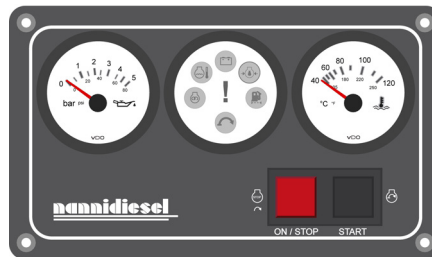
Nanni Deluxe generatorset paneel
